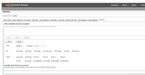
Schedule setup
